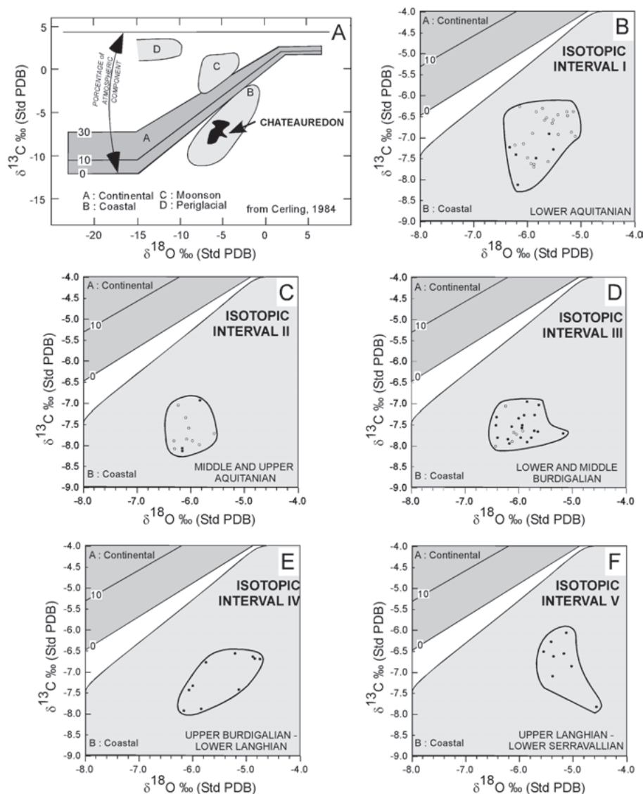
Fig. 7. Cross-diagrams \delta^{18}\text{O}/\delta^{13}\text{C} for paleoenvironmental reconstruction (modified from Cerling, 1984; open dots: BE section; back dots: RU and GR sections).
