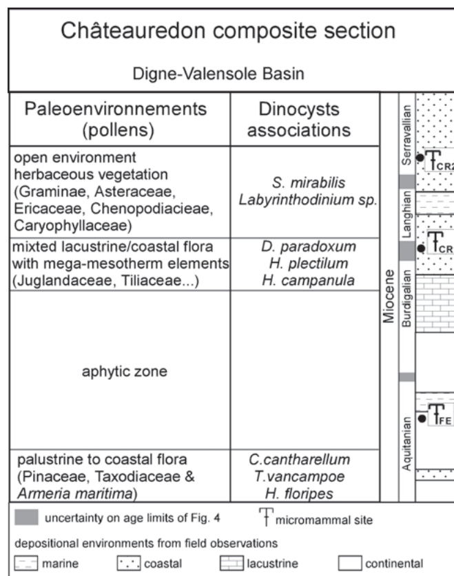
Fig. 6. Paleoenvironmental reconstruction based on pollen and dinocysts associations.
