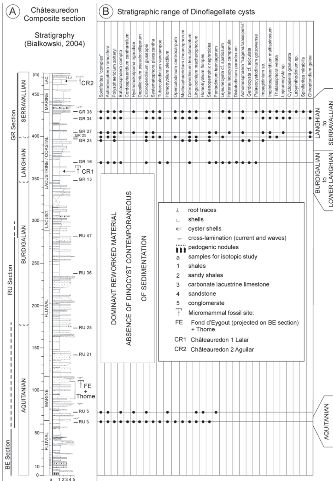
Fig. 2. Composite section of Châteauredon and palynological results
