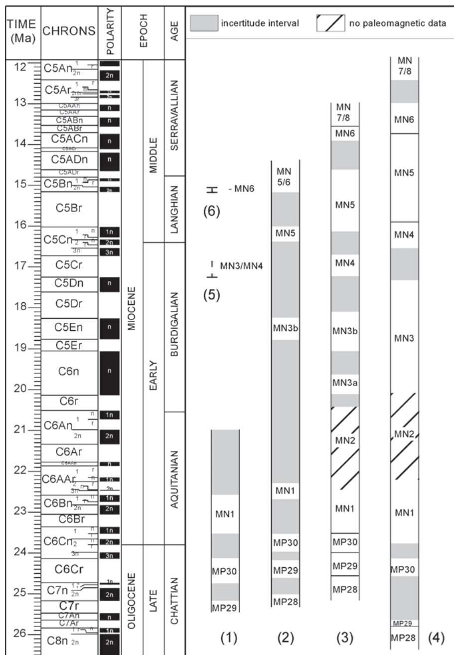
Fig. 5. Correlations of the micromammal biozones to the geomagnetic polarity time scale (1. Burbank et al., 1992; 2. Schlunegger et al., 1996; 3. Kempf et al., 1997; 4. Agusti et al., 2001; 5. Sen, 1997; 6. Aguilar et al., 2003).
