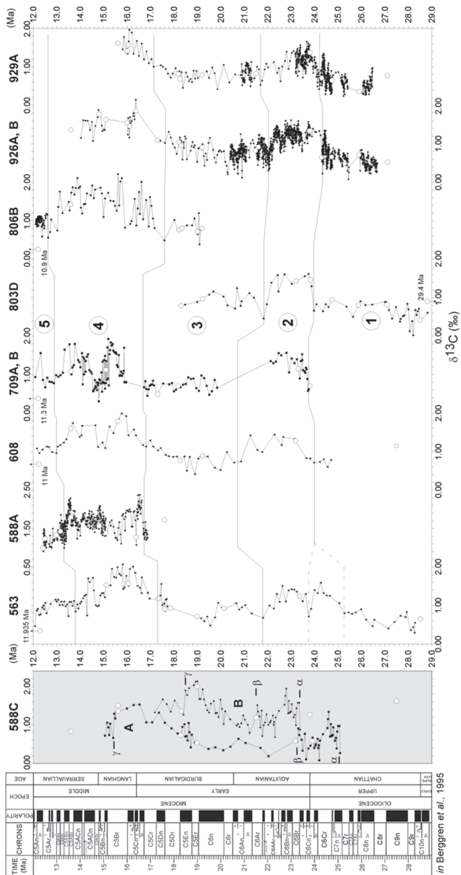
Fig. 3. Variability of the marine carbon isotopic signal, from different DSDP and ODP sites. (open dots – age models). Two different age models are presented for site 588C that is not well calibrated. \alpha , \beta , \gamma are selected points which illustrate the differences between the two stratigraphic calibrations (Lohman, 1986, Martini, 1986, for model A and Kennett 1986, Kennett et al., 1986, for model B).
