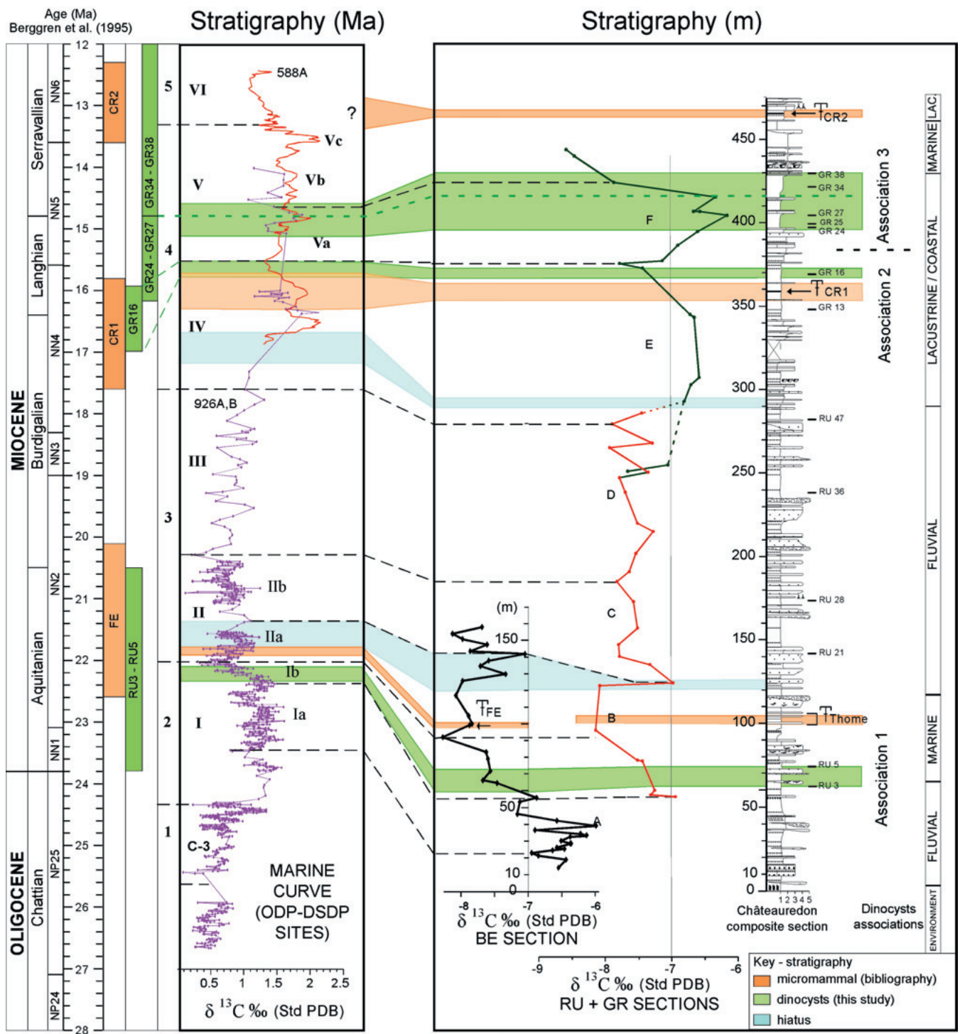
Fig. 4. Integrated stratigraphy of the composite section of Châteauredon (stratigraphy in meters) and correlations to marine data from ODP-DSDP sites recalibrated according to Berggren et al., 1995 (stratigraphy in Ma). Lithologic column, see Fig. 2a,b for key.
