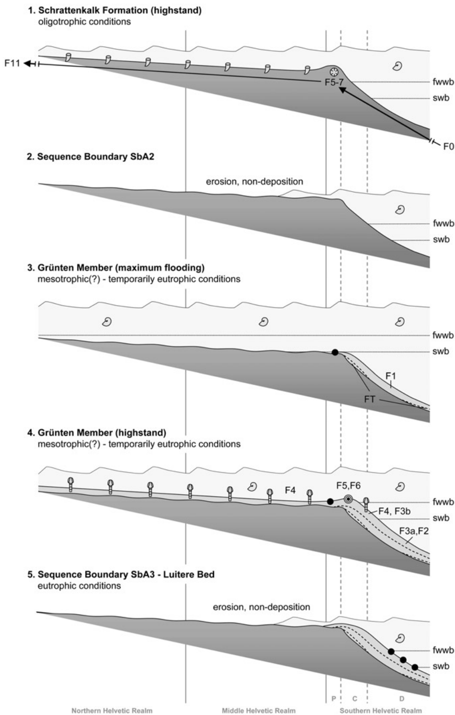
Fig. 10. Speculative, highly simplified schematic sequence depicting the demise of the Urgonian Carbonate Platform and the subsequent installation of the Grünen Ramp. Microfacies codes follow the nomenclature of Arnaud-Vanneau (2005; cf. microfacies codes in Fig. 9); the arrows mark the microfacies trends in the underlying Urgonian Carbonate Platform. The hatched horizontal lines mark the storm wave base and the fair weather wave base, the vertical dashed lines mark the proximal, central and distal parts of the Southern Helvetic Zone. Black dots mark spots with local phosphogenesis.
