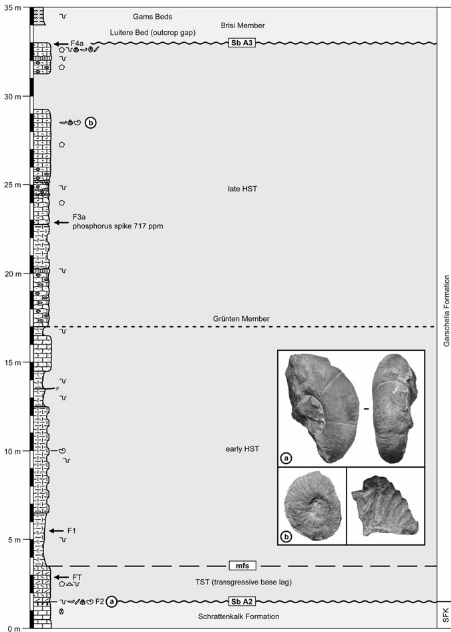
Fig. 4. Profile of the Grünten Member at the lectostratotype section of Morschfeld, Central Switzerland. Inset: A) Pseudohaploceras cf. matheroni (D'ORBIGNY) from the basal firmground (1/3 original size); B) two specimens of Dufrenoyia (?) sp. from the crinoidal upper part of the section (2/3 original size, respectively original size). Photos: M. Delamette. See also Fig. 6 for outcrop photos and Fig. 8 for lithologic symbol key.
