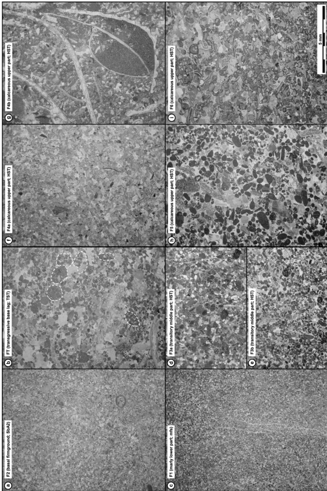
Fig. 7. Thin section photographs of typical microfacies types from the Grünten Member, given in the order of their stratigraphic succession (cf. microfacies codes in Fig. 9). Samples e, h and i are from the Huserstock section (Fronalpstock area, Central Switzerland), g is from the Gütsch section (Bauen-Brisen area, Central Switzerland), all other samples are from the lectotype section of Morschfeld (Bauen-Brisen area; cf. Fig. 2). All photos are given at the same scale (roughly 7x). The dashed lines in photo b mark extraclasts.
