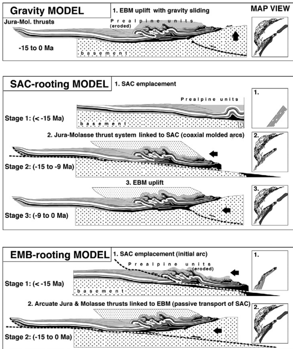
Fig 3. Schematic representation of three models for the kinematics of deformation in French External Alps: view on cross-sections on the left and map-view (in the insets) to the right.
