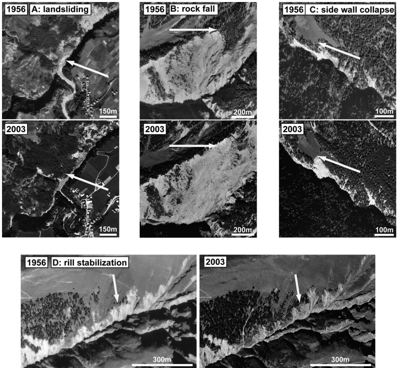
Fig. 5. Comparative orthophoto illustrating examples from the change detection analyses. The arrows mark the location where well-visible changes have occurred. See Fig. 6 for location of examples (squares labelled with A, B, C and D). Reproduced with permission from Swisstopo (BA091200).
