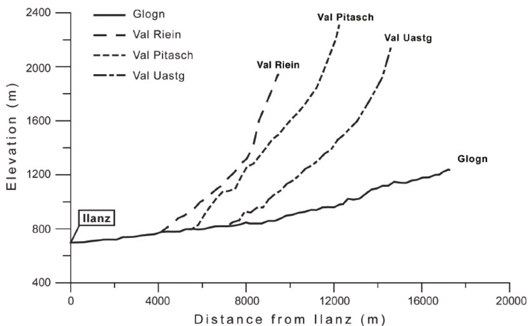
Fig. 4. Morphometric properties of the Glogn valley and longitudinal stream profiles of the Glogn and tributary rivers. The Lumnezia landslide shows a significantly lower roughness magnitude (mean) and standard deviation (StDev) than the three deeply incised valleys on the eastern side of the Glogn. Steps in stream profiles reflect raster points in the DEM. See text for further explanation. Reproduced with permission from Swisstopo (BA091200).
