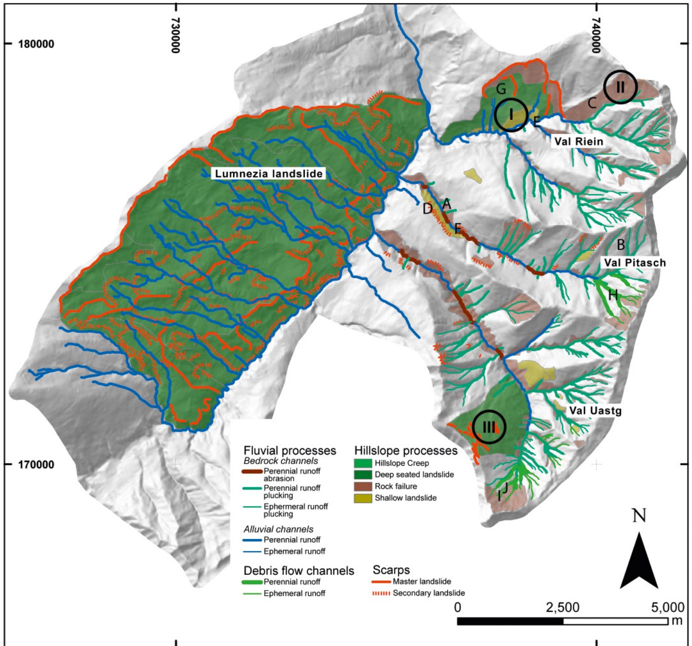
Fig. 3. Geomorphological map representing the situation in 2003. Specific sites are described in the text. The channel floors of alluvial channels are covered by a sedimentary layer and thus contrast to bedrock channels that have been shaped by abrasion and plucking. A–J are sites of photos illustrated on Figure 2; I, II and III are sites of landsliding in the eastern tributary catchments. Reproduced with permission from Swisstopo (BA091200).
