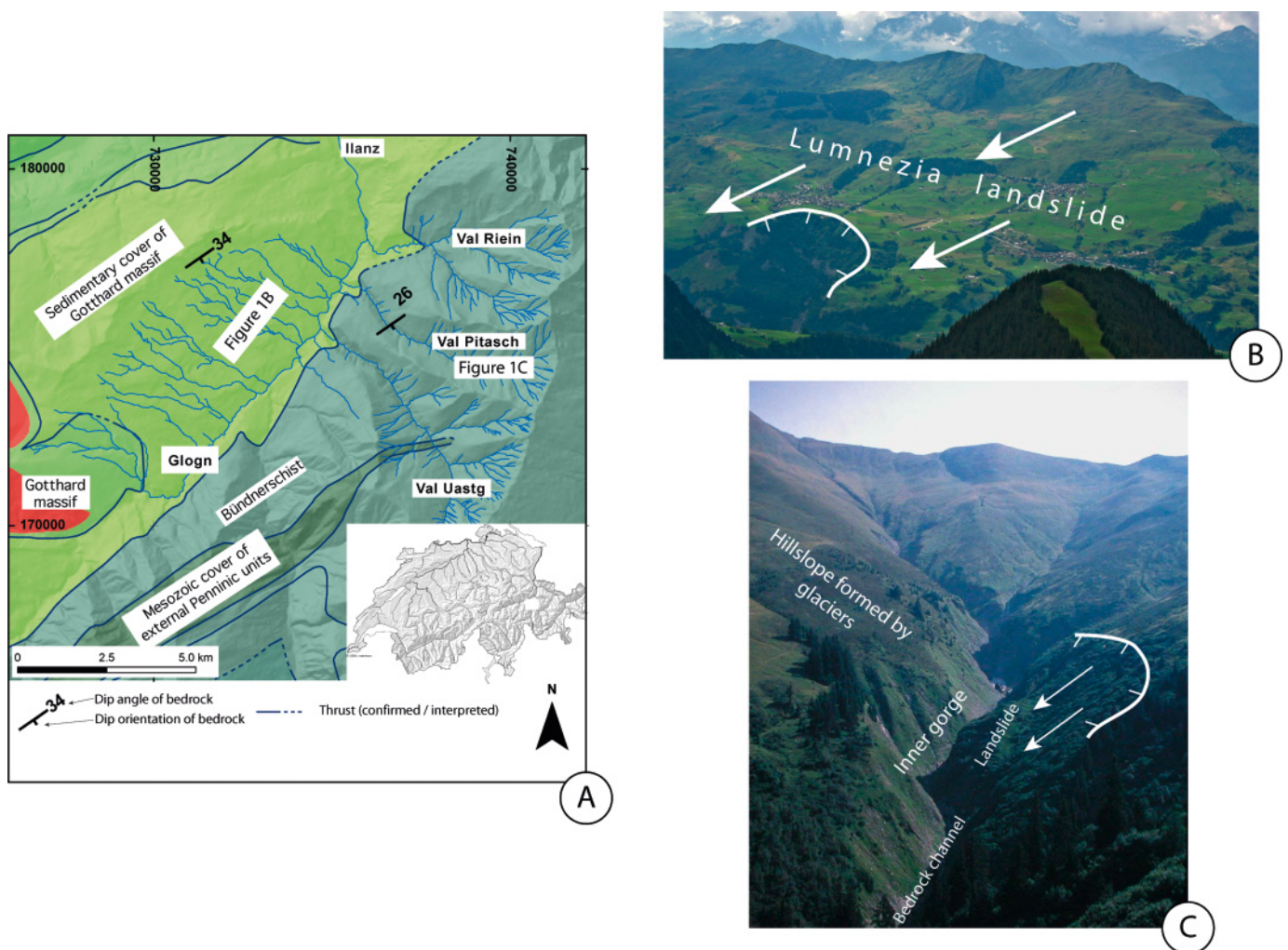
Fig. 1. (A) Geological map of the Lumnezia area, south of Ilanz. Source according to Spicher (1984). The inset shows the location of Val Lumnezia. The thrust between the Bündnerschists and the Mesozoic cover of the Gotthard Massif (Misox zone) runs parallel to the Glogn River. (B) and (C) are photos from the western and eastern valley sides. See text for further explanation. Reproduced with permission from Swisstopo (BA091200).
