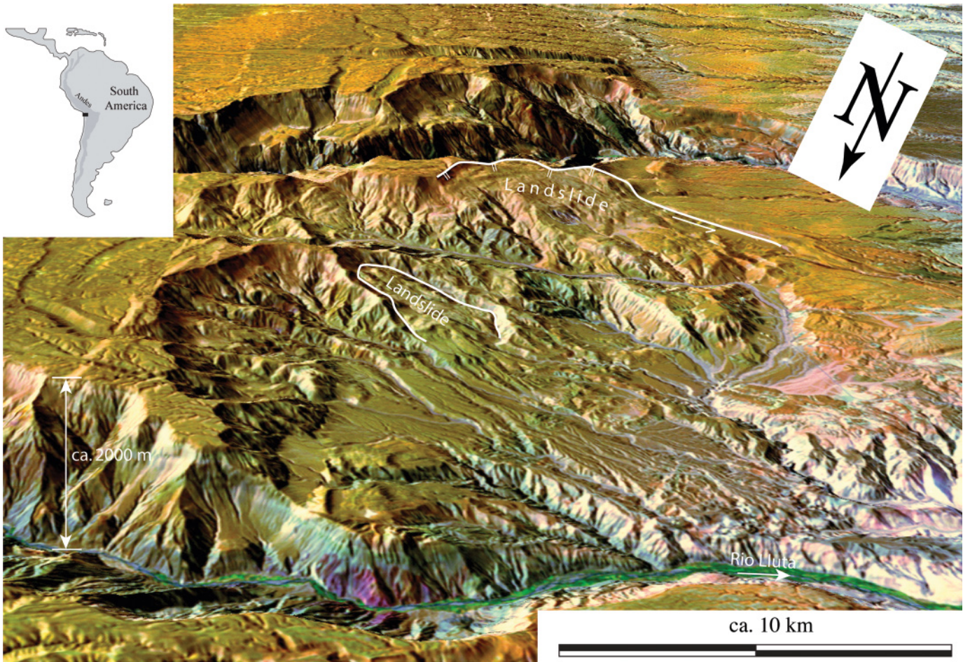
Fig. 7. Example of a landscape in northern Chile where landsliding has inhibited the establishment of a channel network. The Lluta collapse evolved as response to initial landsliding that removed a total of 26 km 3 of mass (Strasser & Schlunegger 2005). Subsequence modification of the landslide scar occurred by headward erosion, resulting in the establishment of a dendritic drainage network and the removal of an additional 24 km 3 of mass. The age of the initial landslide is >2.5 Ma (Schlunegger et al. 2006).
