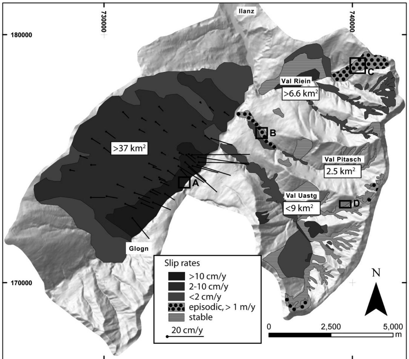
Fig. 6. Areas that have delivered material to the channel network between 1959 and 2003. A–D represent sites with obvious topographic changes detected on aerial photographs (Fig. 5). Note that landscape changes need to exceed 1 m in order to be detected on aerial photographs (see also Schwab et al. 2008). Reproduced with permission from Swisstopo (BA091200).
