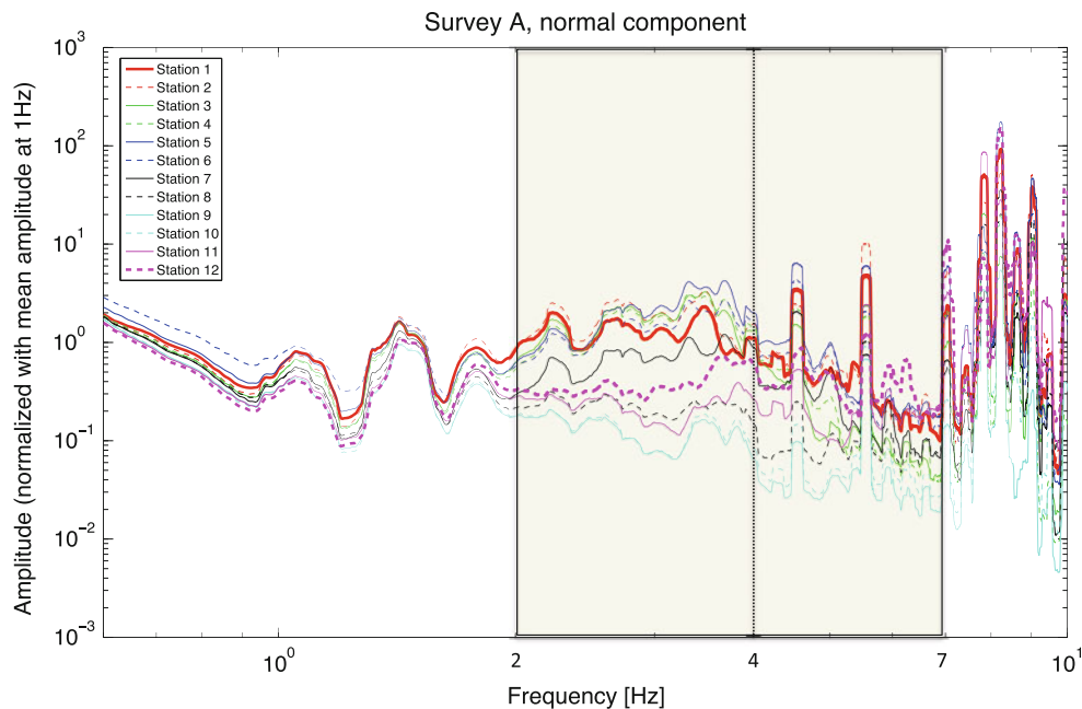
Fig. 3 Ambient vibration survey data: normalized amplitude as a function of frequency (0.6–10 Hz) of Survey A (normal component, i.e. horizontal and perpendicular to the trace of the assumed fault). Each line represents a trace of a seismic station. At low frequencies (<2 Hz), the motion is about the same in all stations. For frequencies in the range between 2 and 7 Hz (yellow box), the signals are significantly different. For frequencies larger than 7 Hz, the signals are more or less consistent again
