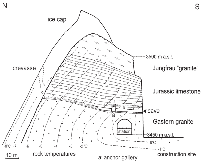
Fig. 1. Geological cross section of Jungfrauoch-Sphinx (after Keusen & Amiguet 1987). Karst cave with unknown extension to the north.
