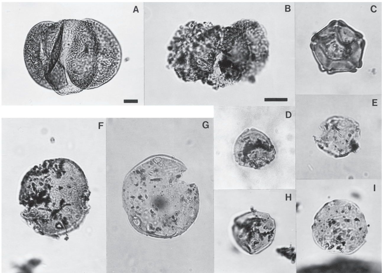
Fig. 4. Examples of pollen from Jungfrauoch cave sediments. (A–B) Pinus , sample no. 1; (C, E) Alnus , no. 7; (D) Triporate indet., no. 1; (F) Tilia , no. 7; (G) Carya , no. 2; (H) Triporate indet., no. 7; (I) Ulmus , no. 7. Scale = 10 \mu\text{m} ; note different scale for A.
