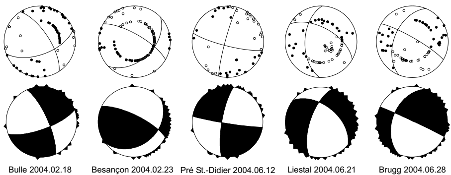
Fig. 4. Faultplane solutions (above) based on first-motion polarities and moment tensors (below) based on full-waveform inversion (lower hemisphere, equal area projection). In the faultplane solutions, solid circles correspond to compressive first motion (up) and empty circles to dilatational first motion (down); on the moment tensors, triangles show the station locations.
